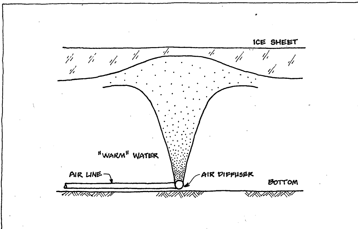
FIGURE 8.1: Compressed Air Ice Suppression System (after Ashton 1974)
