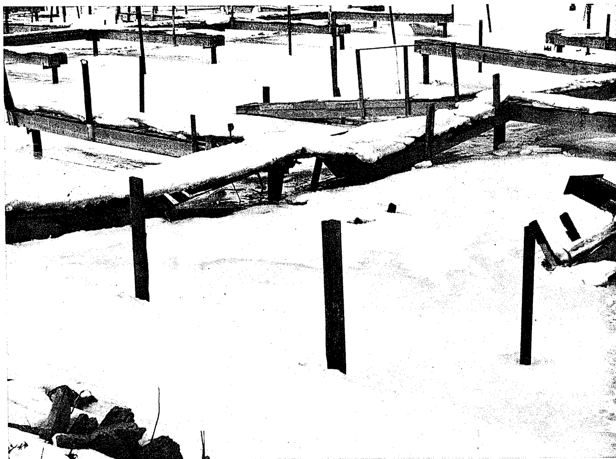
FIGURE 6.5: Marina Piers Damaged by Ice Movement with River Stage Changes
