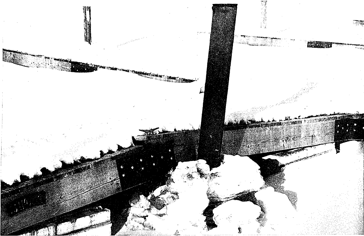
FIGURE 9.5: Floating Dock Damaged by Lifting Pile
