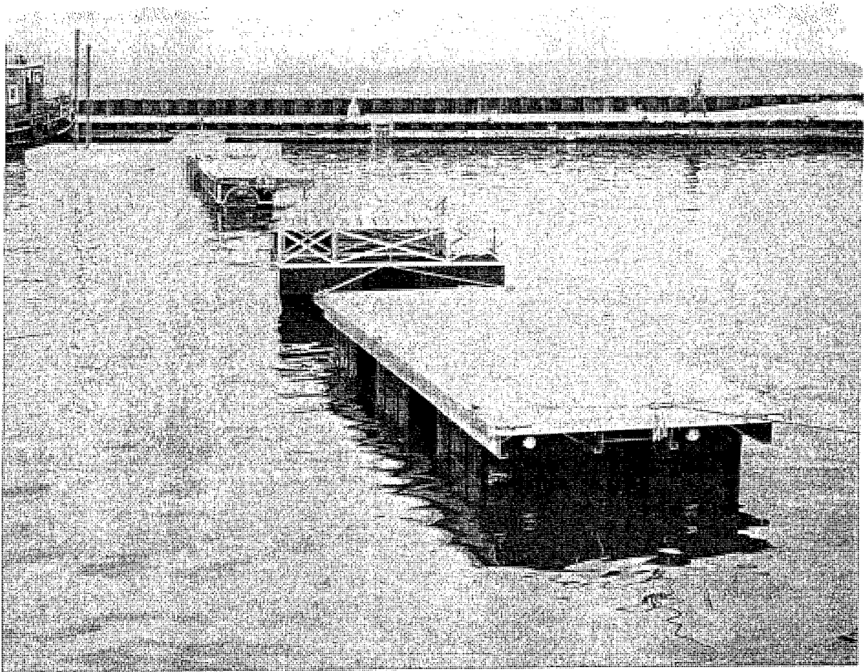
FIGURE 9.3: Floating Docks in Bayfield, Wis., Harbor Test
