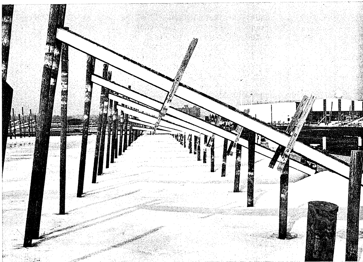
FIGURE 7.2: Damage to "Unprotected" Dock
