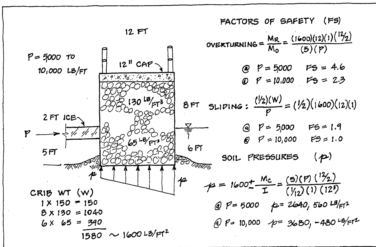
FIGURE 10.2 Analysis of Crib with Ice Thrust
