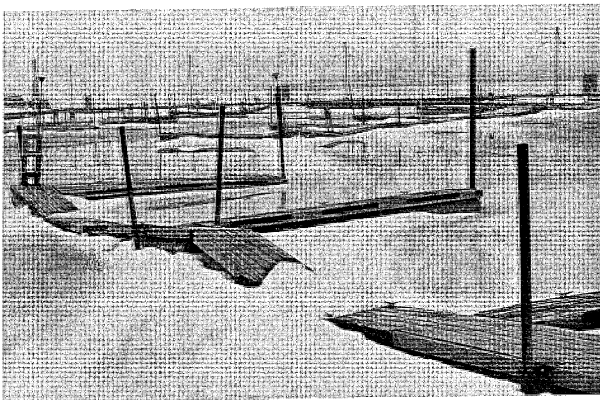
FIGURE 9.7: Floating Dock Contorted by Ice
