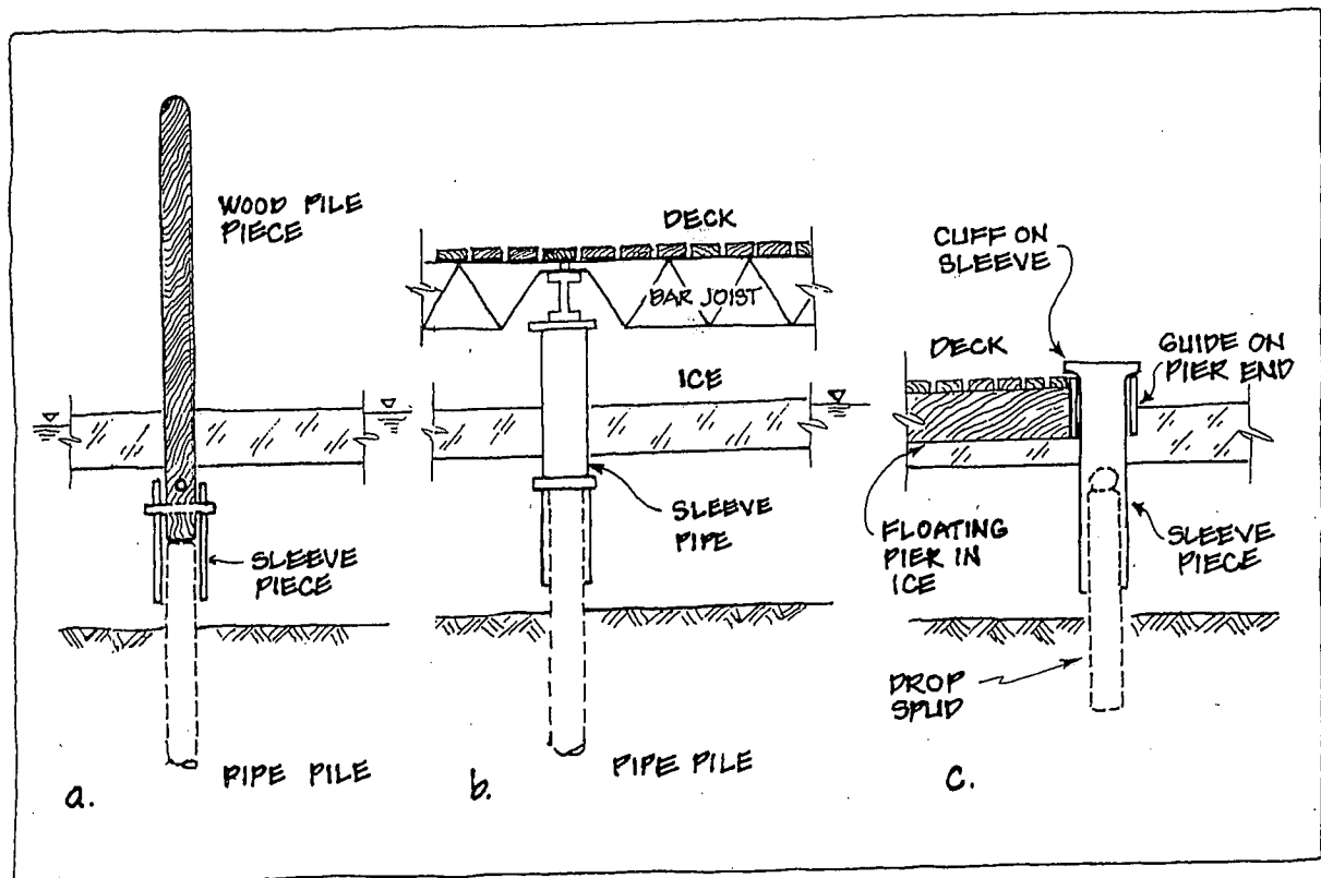
FIGURE 11.3: (a) Sleeved Mooring Pile (b) Sleeved Dock Pile (c) Sleeved Drop Spud
