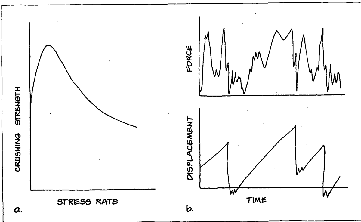
FIGURE 3.4b: Force and Displacement vs. Time Plots
