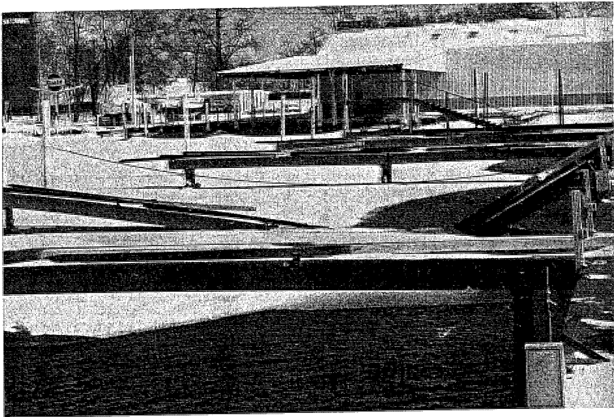
FIGURE 7.1: Damage to "Deiced" Dock
