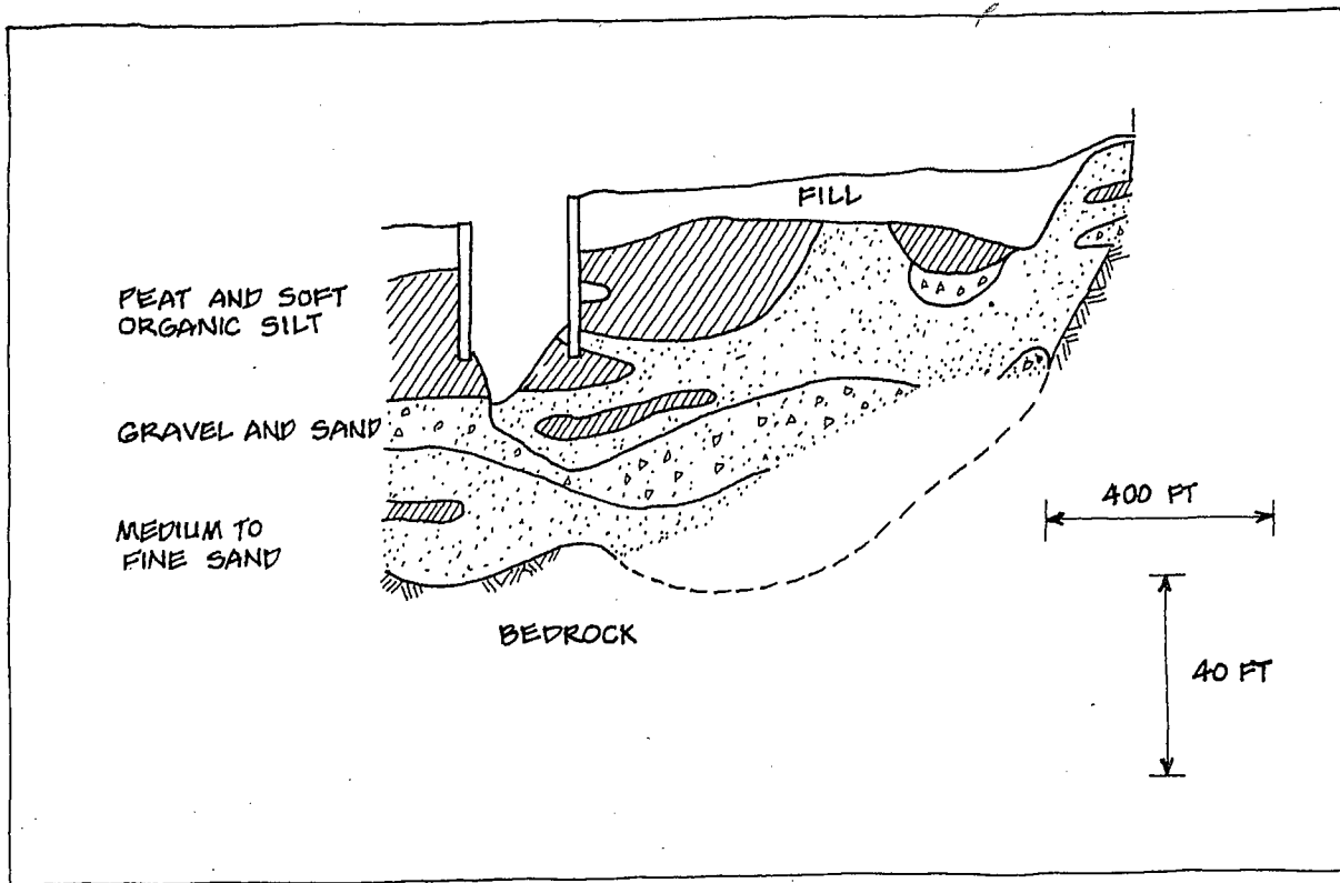
FIGURE 6.2: Cross Section of Composite Shore Deposit Near Mouth of the Milwaukee River, Wisconsin. (after Peck et al. 1975)
