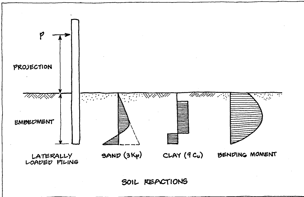
FIGURE 12.1: Laterally Loaded Piling, Soil Reactions and Bending Moments (after Broms)
