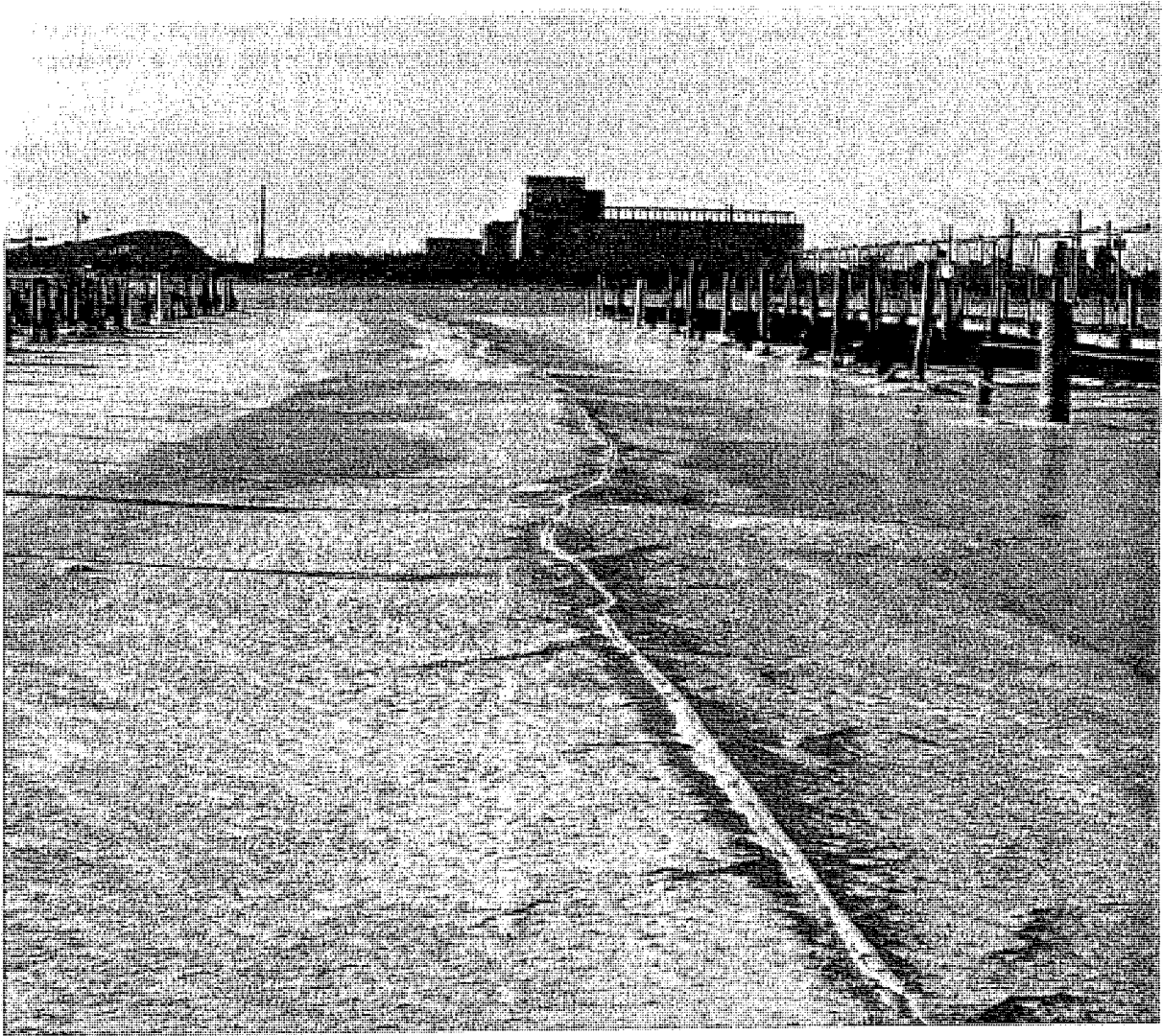
FIGURE 3.7: Thermally Active Ice Sheet Aisle Crack Buckled Between Head Piers
