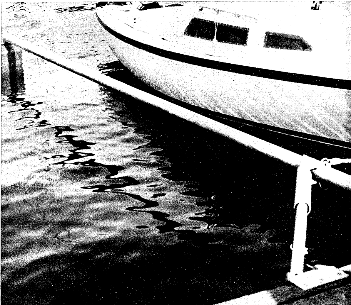
FIGURE 9.11: "Shock Absorber" Mooring Arm
