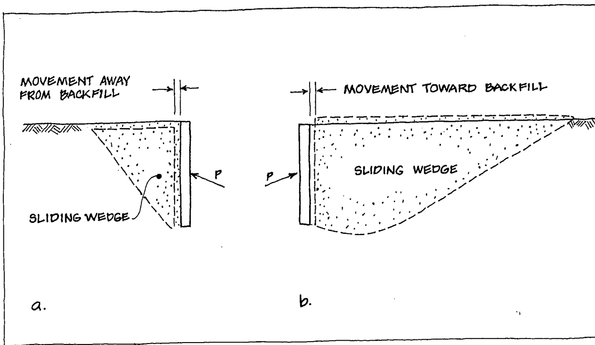
FIGURE 5.2a: Active Earth Pressure. 5.2b: Passive Earth Pressure. (after Teng 1962)
