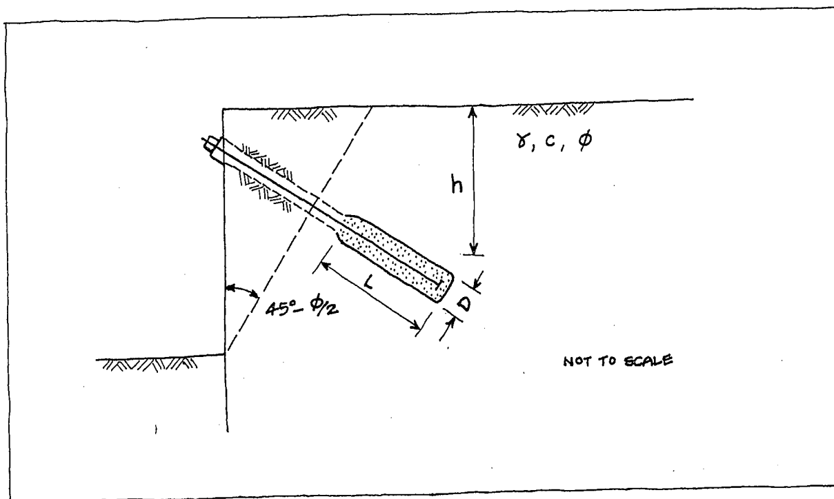
FIGURE 5.3: Grouted Tieback Anchor in a Drilled Hole.
