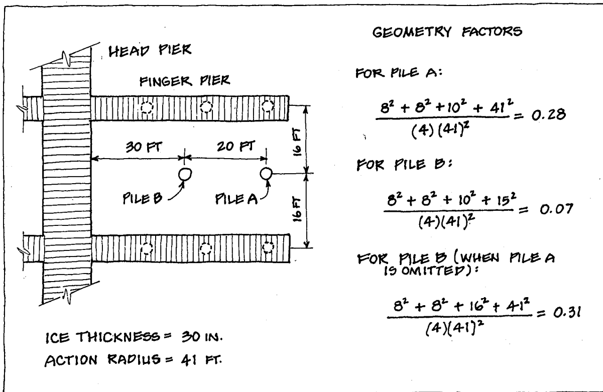
FIGURE 11.9: Example Calculations of Geometry Factors (after Roblee 1983)
