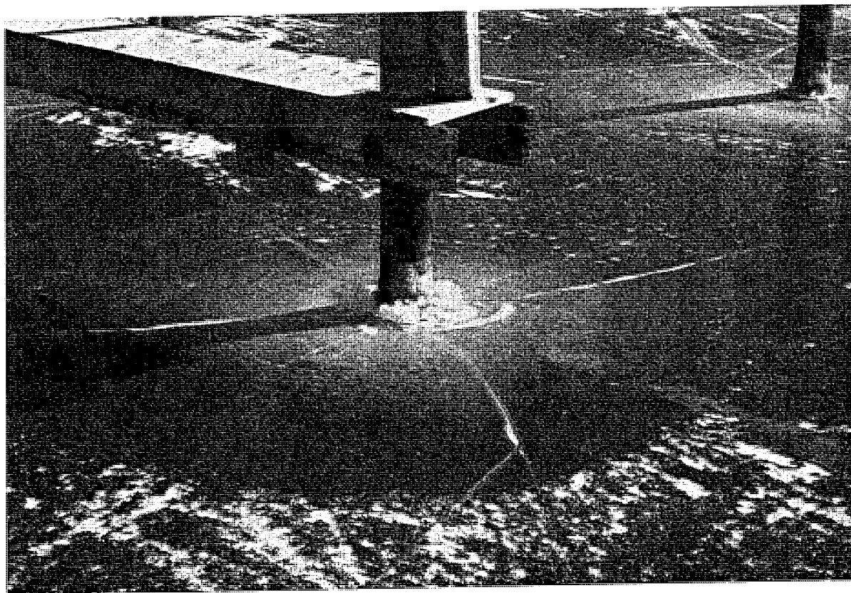
FIGURE 3.2: Thin Ice Cracking on a Steel Piling
