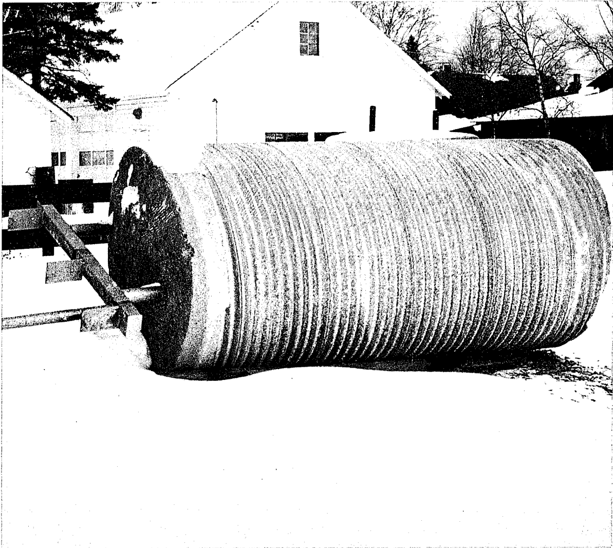
FIGURE 5.4: "Failed" Steel Cell Canister Structure.
