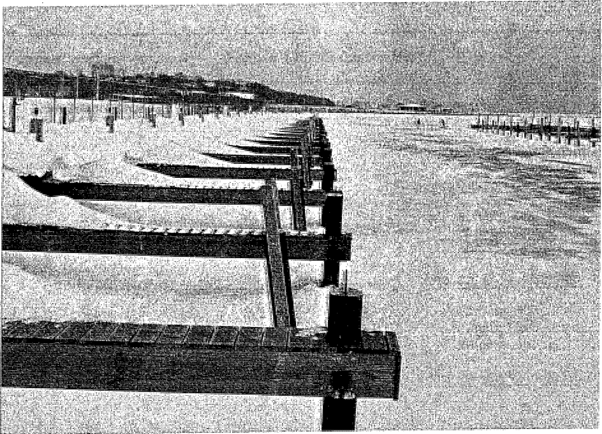
FIGURE 12.2: Free-Standing Mooring Piles Permanently Deflected by Ice in a Confined Harbor Basin
