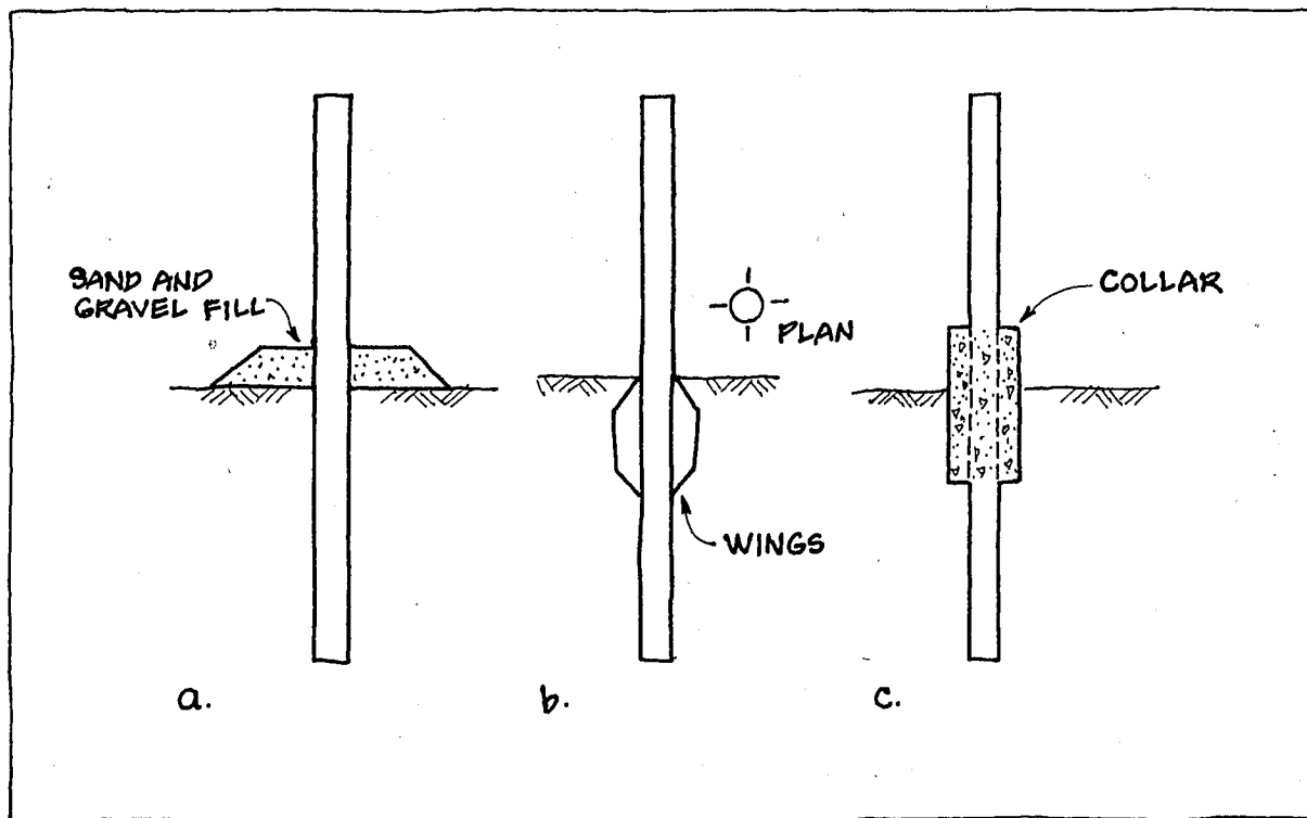
FIGURE 12.3: Methods Used to Increase the Lateral Resistance of Piles (after Broms 1972)
