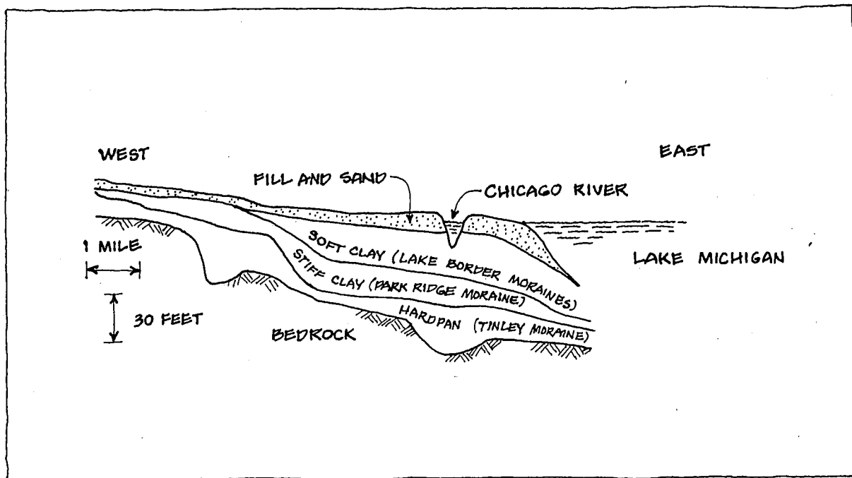
FIGURE 6.1: Simplified Cross Section of Glacial Deposits beneath Lake Street in Chicago: Successive Ground Moraines. (after Peck et al. 1974)
