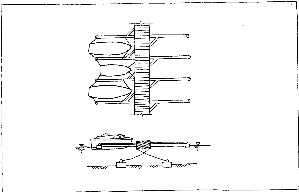
FIGURE 9.10: Floating Dock with Mooring Arms (after the Swedish guide Home Harbors for Leisure Boats by W. Altrock)
