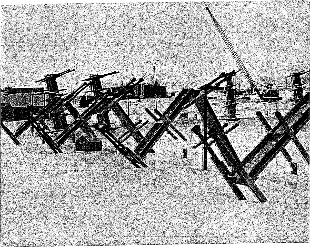
FIGURE 7.6: Fixed Piers Hinged for Winter Removal
