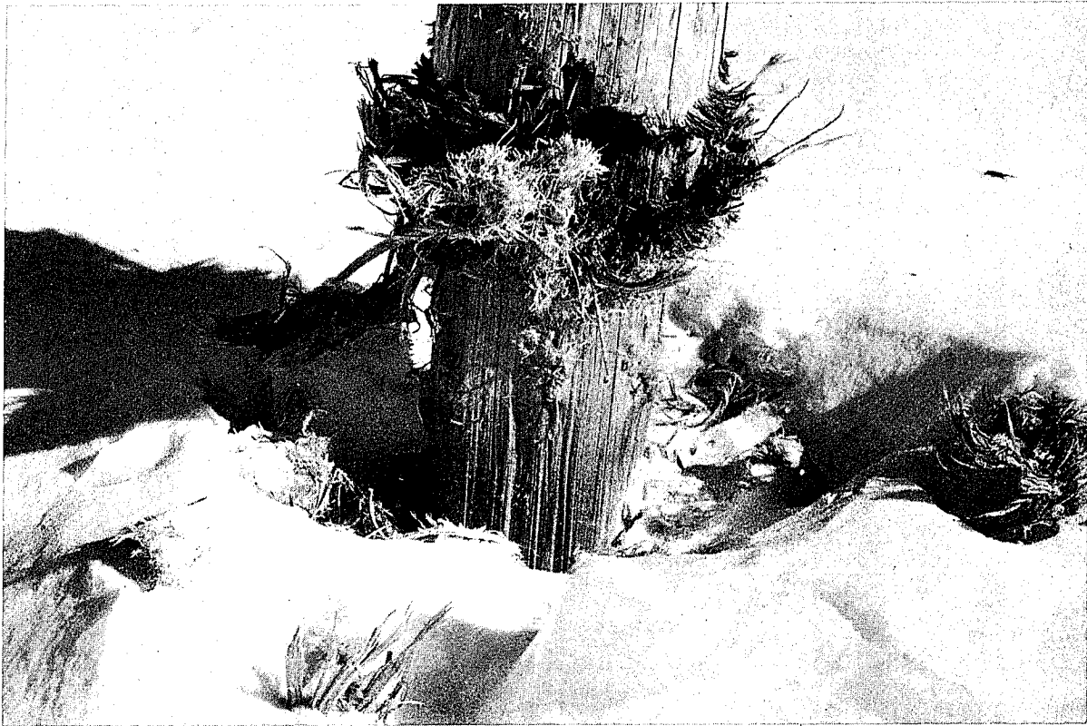
FIGURE 11.6: Untreated Timber Pile Being Shredded by Ice
