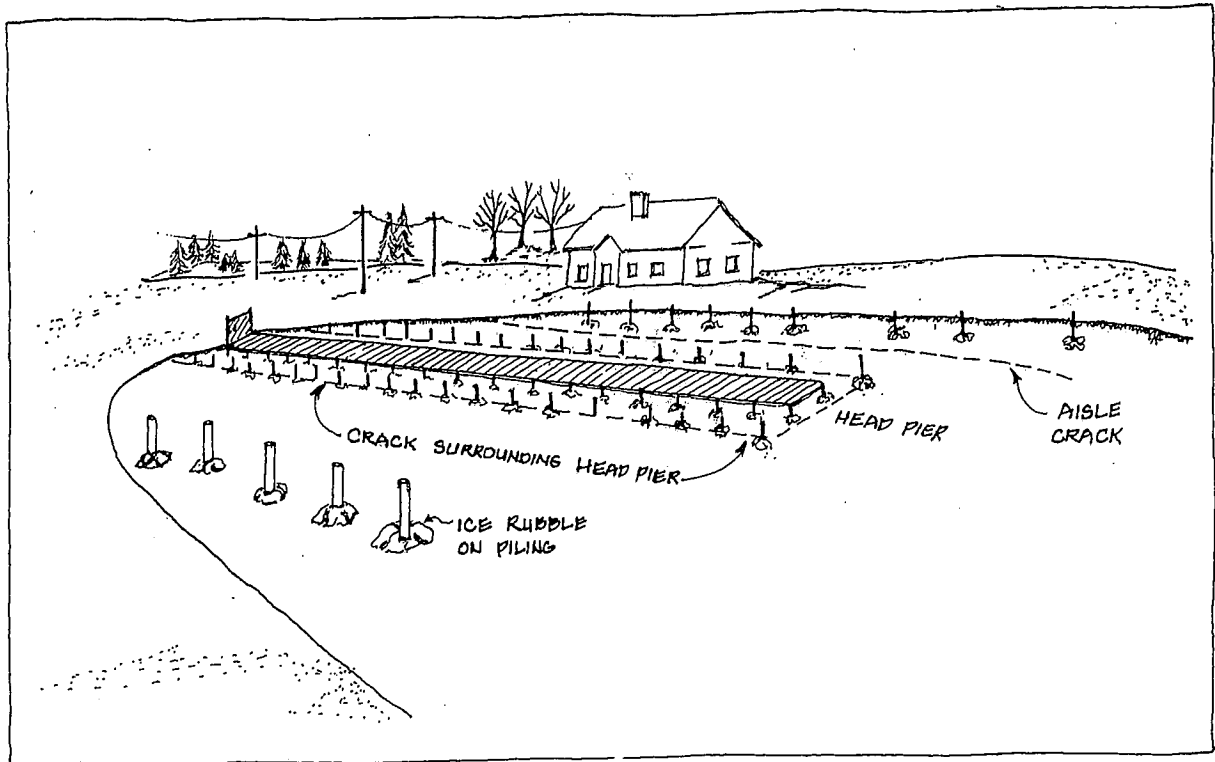
FIGURE 11.7: Group Action Cracking of Ice Sheet Around Head Pier
