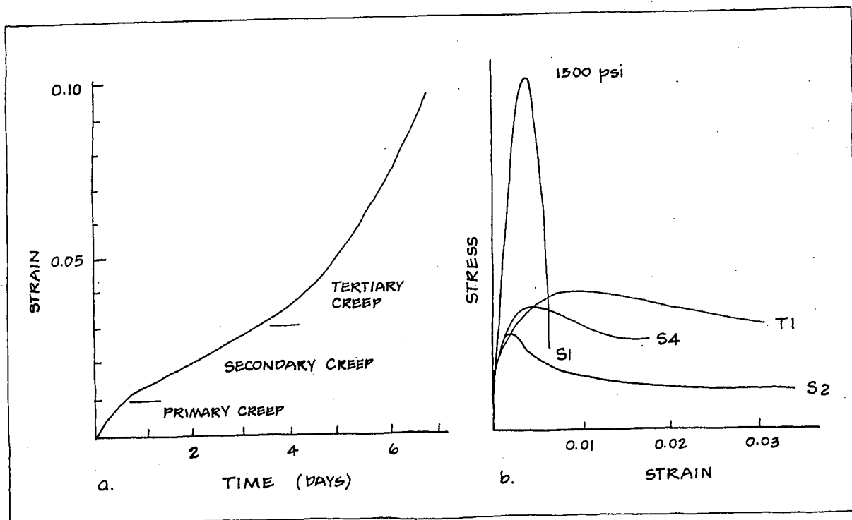
FIGURE 3.1a: Creep Curve for Granular Ice 3.1b: Strain Dependence on Stress (after Gold 1973)
