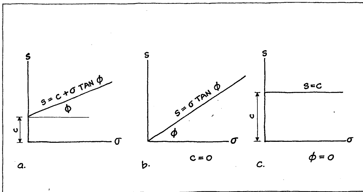
FIGURE 4.1: Mohr-Coulomb strength criterion for (a) c - \phi soil, (b) \phi -soil (cohesionless) and (c) c -soil (cohesive).
