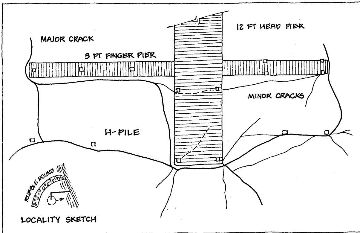
FIGURE 11.8: Group Action at End of L-shaped Pier
