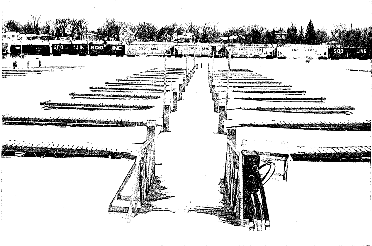
FIGURE 7.4: Floating Docks Wintering in a Quiet, Well-Protected Harbor
