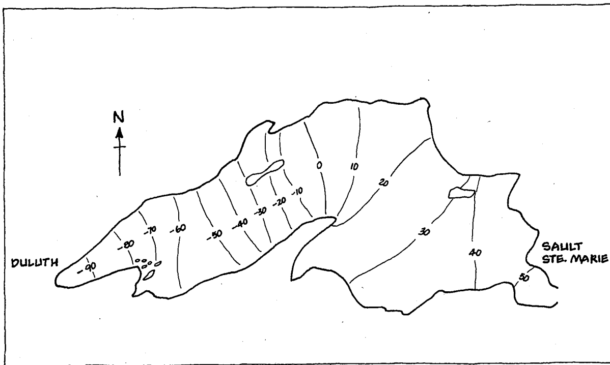
FIGURE 6.4: Basin Oscillations, First Mode, Lake Superior Contour 100 = about 43 inches. (after Rao and Schwab 1976)
