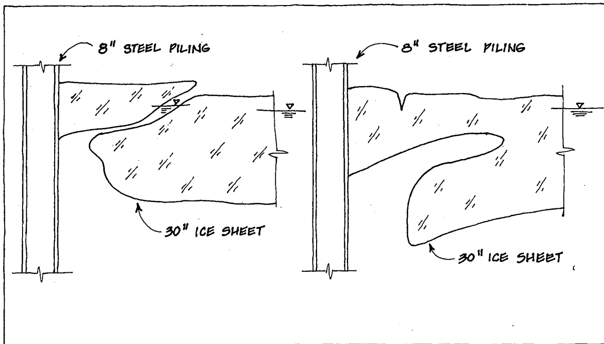
FIGURE 6.7: Half Cross Sections of Ice Sheets Attached to Steel Piling
