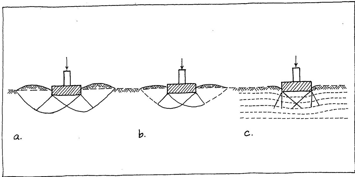
FIGURE 5.1: Modes of Bearing Capacity Failure: (a) General Shear Failure, (b) Local Shear Failure, (c) Punching Shear Failure
