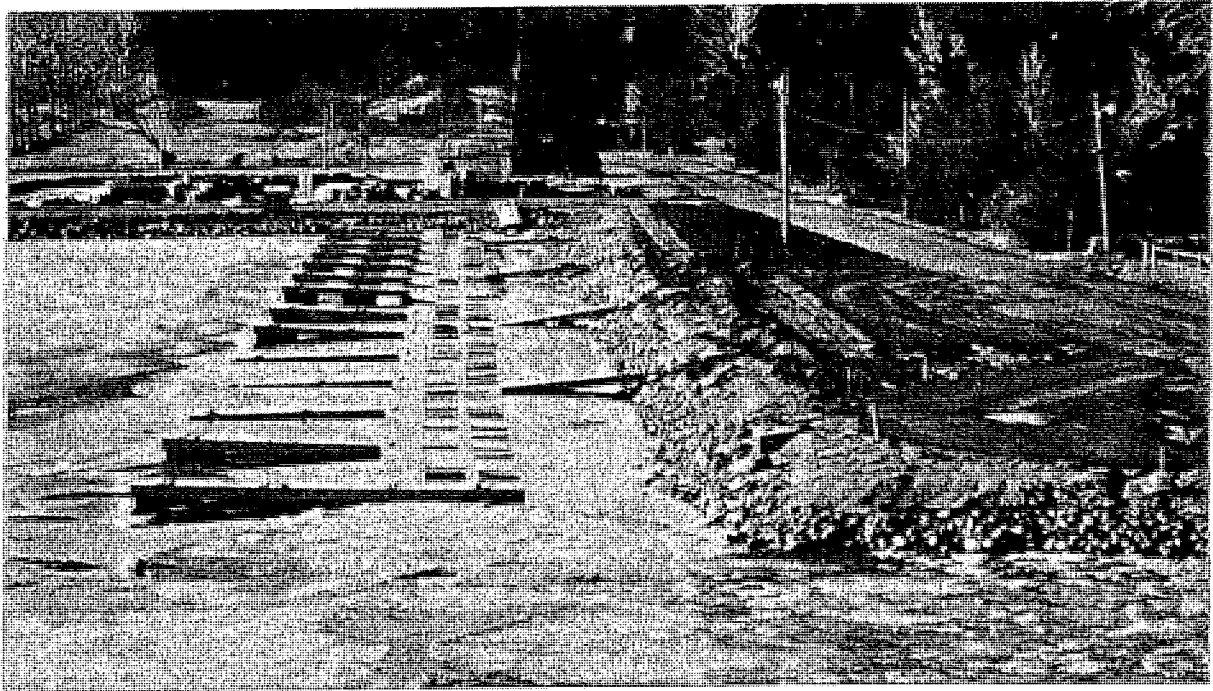
FIGURE 9.1: Hollow (Unfilled) Fiberglass Pontoon System Damaged by Ice
